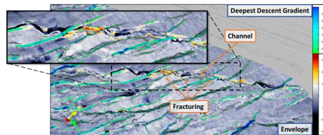
Figure 5: Co-rendering in 3D of the seismic envelope and the Deepest Descent Gradient on a horizon at the reservoir level.
