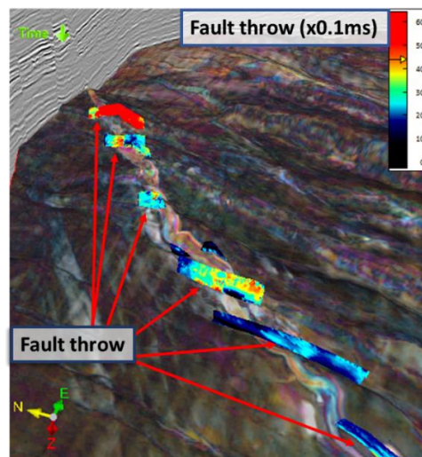
Figure 6: Co-rendering in 3D of spectral decomposition in RGB and the fault throw attribute at the reservoir level.
